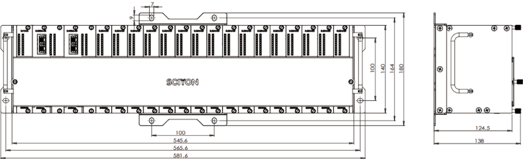
16槽机笼545.6(581.6)mm*180(140)mm*138mm
