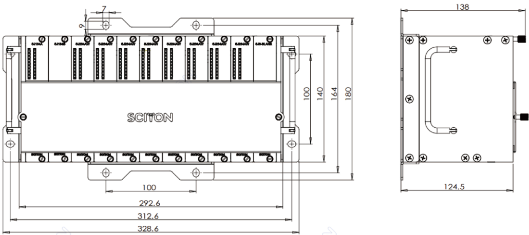
8槽机笼292.6(328.6)mm*180(140)mm*138mm 8槽主机、扩展机笼尺寸大小相同
